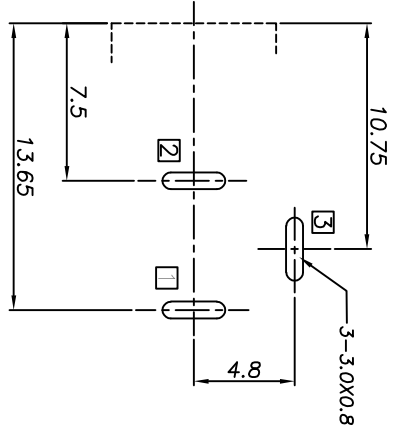
P. C. B Layout (Copper-sided view)
