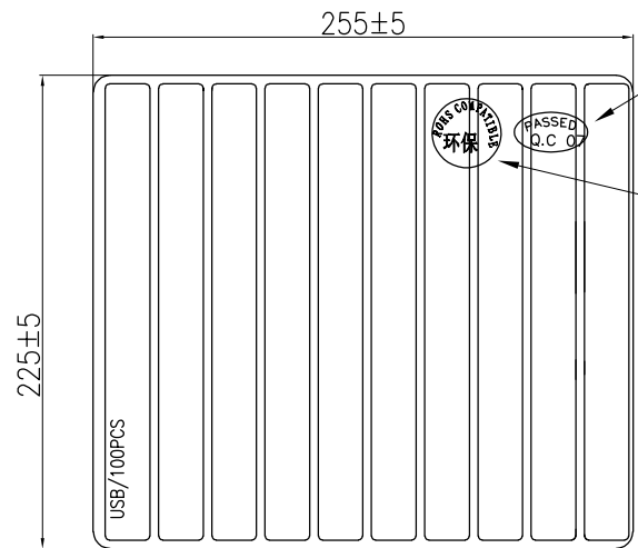
吸塑盒上盖
