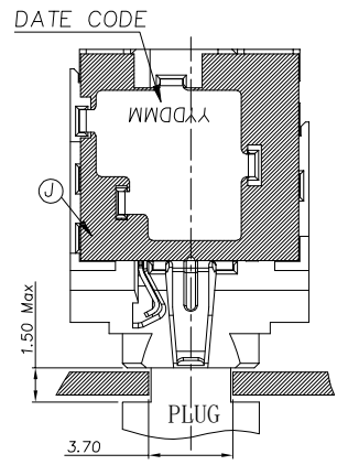
RECOMMENDED PANEL'S ID TOP VIEW; TOL.±0.05
