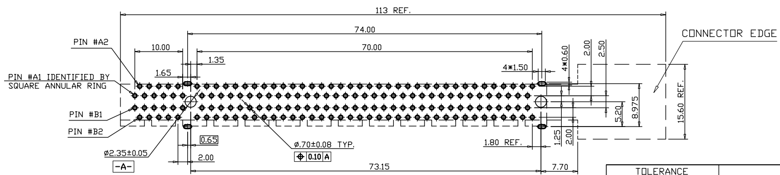
RECOMMENDED PCB LAYOUT <COMPONENT SIDE> TOLERANCE: ±0.05
