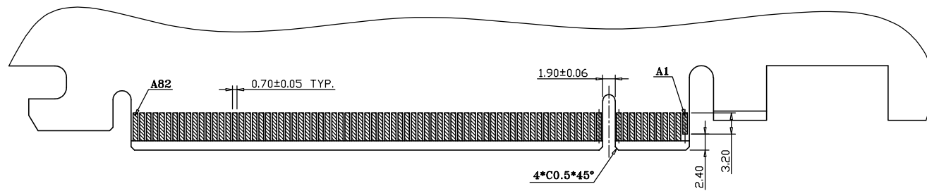
RECOMMENDED EDGE CARD PATTERN<SECONDARY SIDE>
