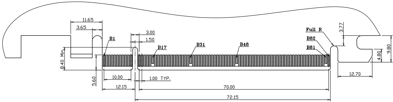
RECOMMENDED EDGE CARD PATTERN<PRIMARY SIDE>
